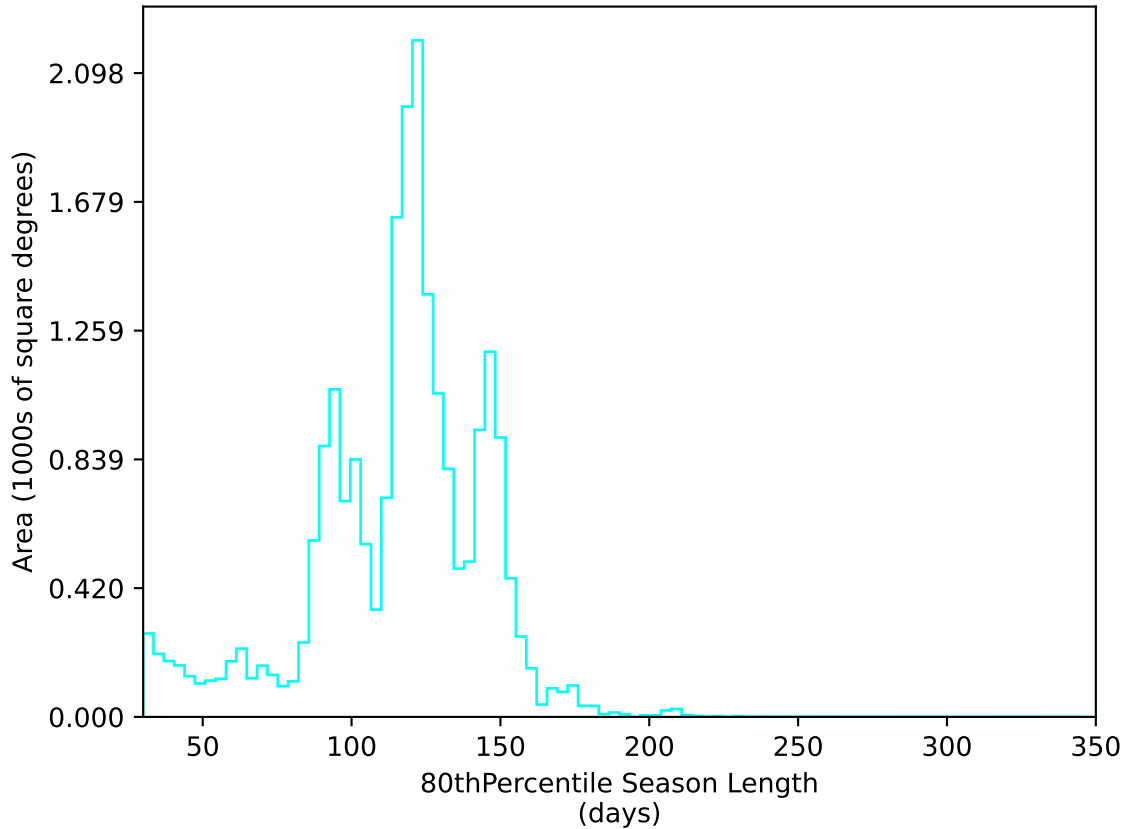
too_elab_heavy_r32_d3_ugrizyv3.4_10yrs All sky u band: 80thPercentile Season Length
