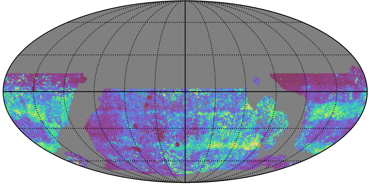
too_elab_heavy_r32_d3_ugrizy_v3.4_10yrs WFD zy bands: 75th Percentile Intranight Timespan
