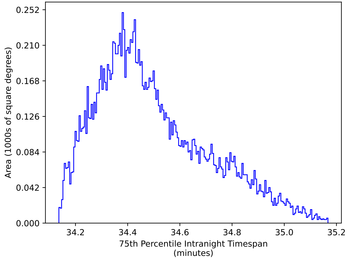
too_elab_heavy_r32_d3_ugrizy_v3.4_10yrs WFD zy bands: 75th Percentile Intranight Timespan
