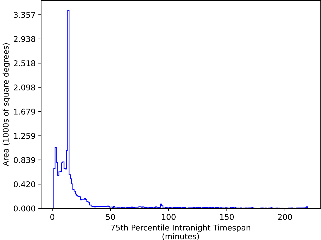
too_elab_heavy_r32_d3_ugrizy_v3.4_10yrs WFD z band: 75th Percentile Intranight Timespan
