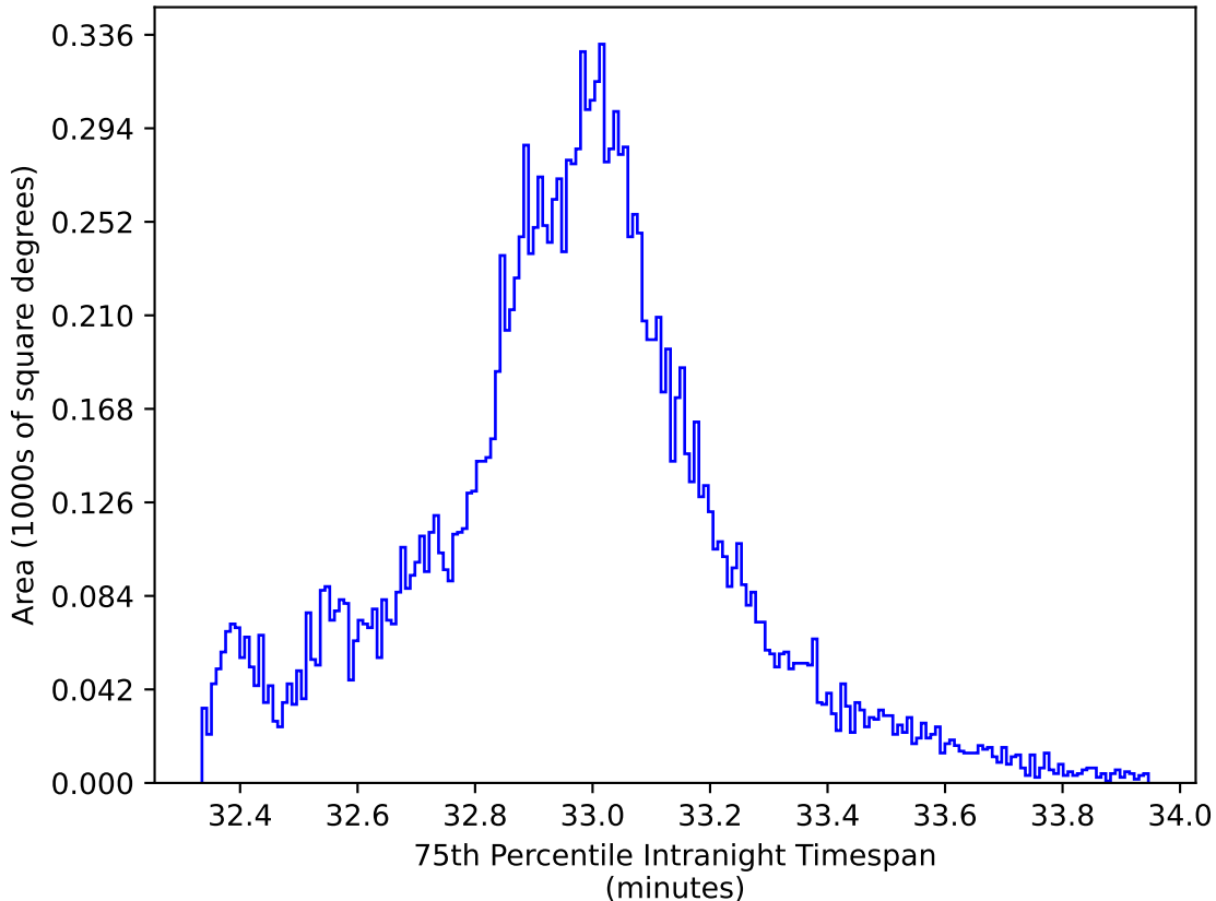
too_elab_heavy_r32_d3_ugrizy_v3.4_10yrs WFD y band: 75th Percentile Intranight Timespan
