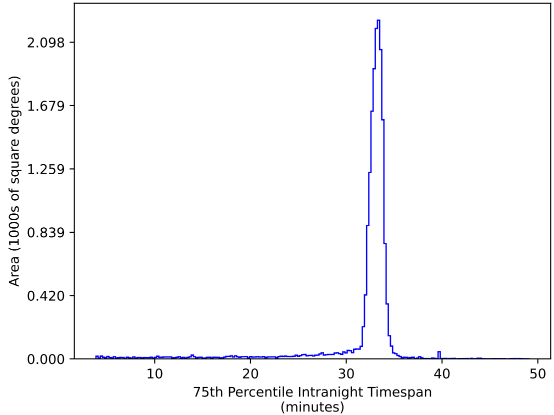
too_elab_heavy_r32_d3_ugrizy_v3.4_10yrs WFD ug bands: 75th Percentile Intranight Timespan
