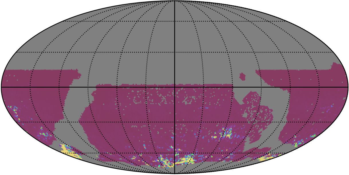
too_elab_heavy_r32_d3_ugrizy_v3.4_10yrs WFD ri bands: 75th Percentile Intranight Timespan
