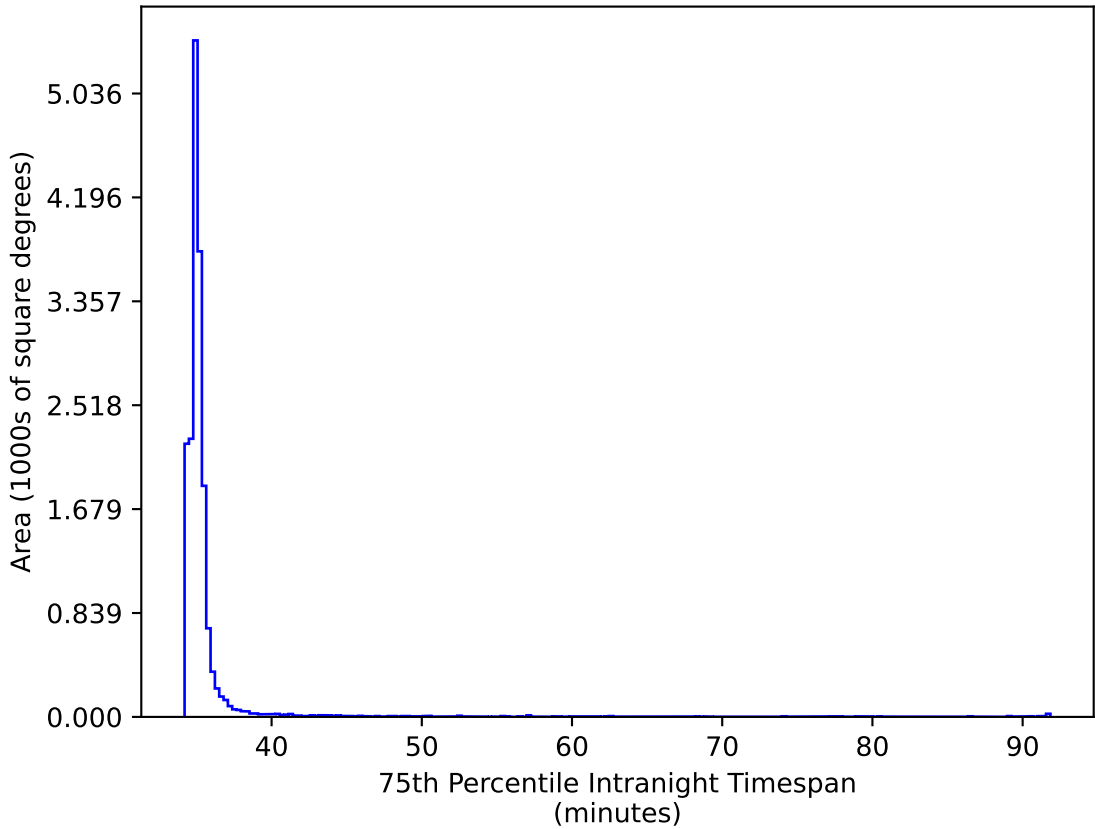
too_elab_heavy_r32_d3_ugrizy_v3.4_10yrs WFD ri bands: 75th Percentile Intranight Timespan
