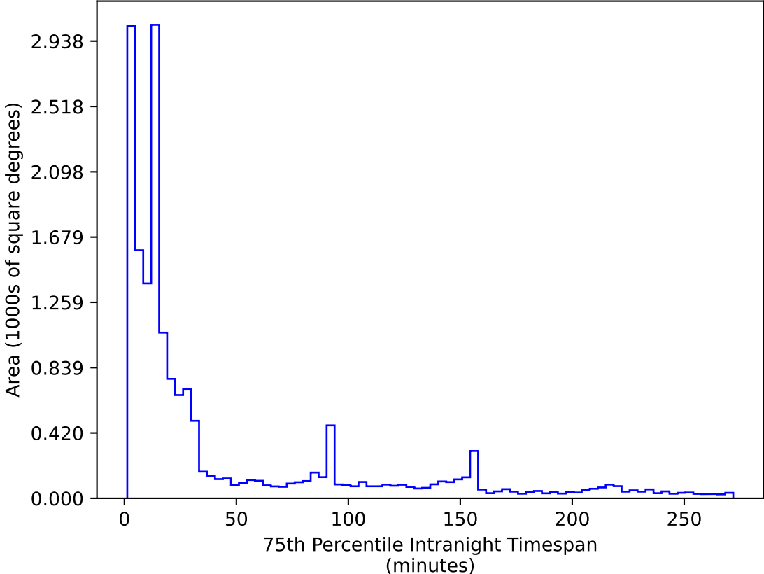
too_elab_heavy_r32_d3_ugrizy_v3.4_10yrs WFD r band: 75th Percentile Intranight Timespan
