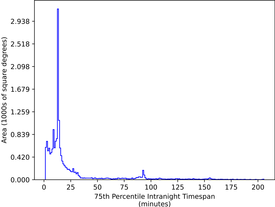
too_elab_heavy_r32_d3_ugrizy_v3.4_10yrs WFD i band: 75th Percentile Intranight Timespan
