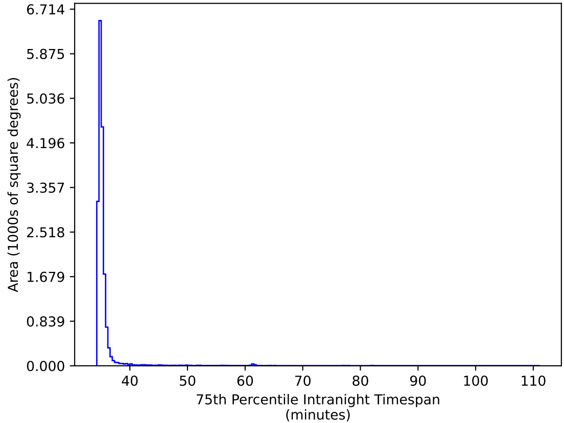
too_elab_heavy_r32_d3_ugrizy_v3.4_10yrs WFD gr bands: 75th Percentile Intranight Timespan
