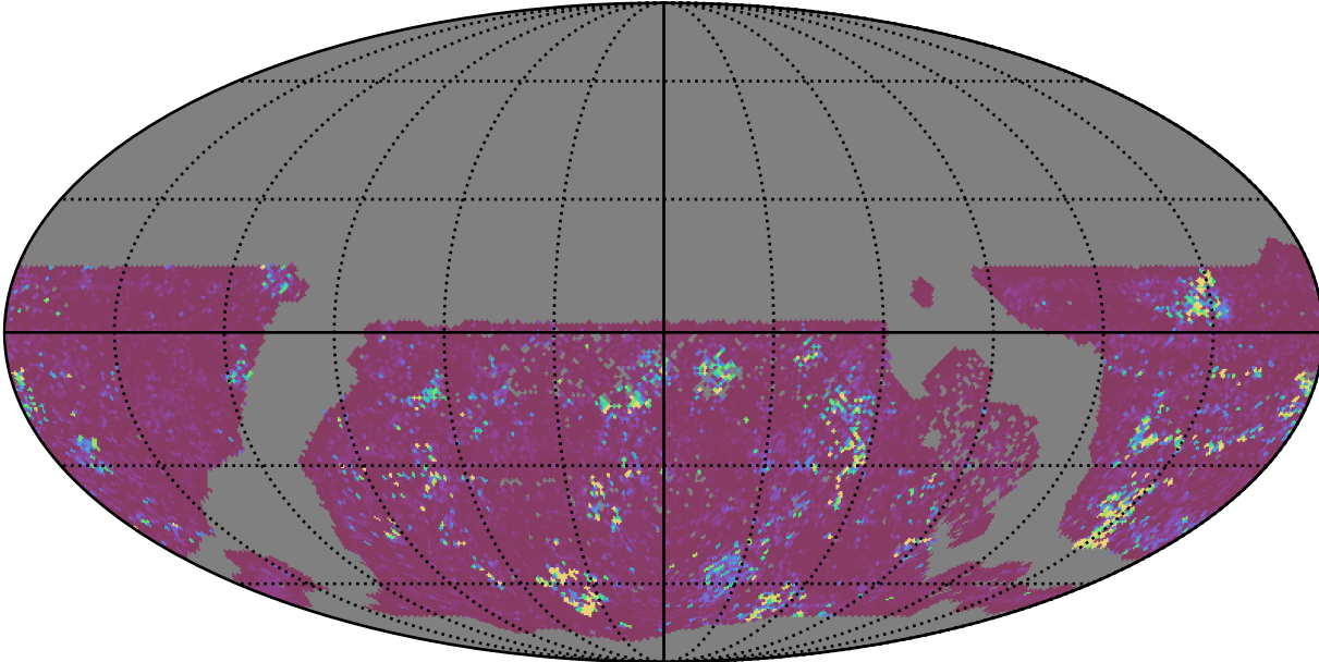
too_elab_heavy_r32_d3_ugrizy_v3.4_10yrs WFD g band: 75th Percentile Intranight Timespan
