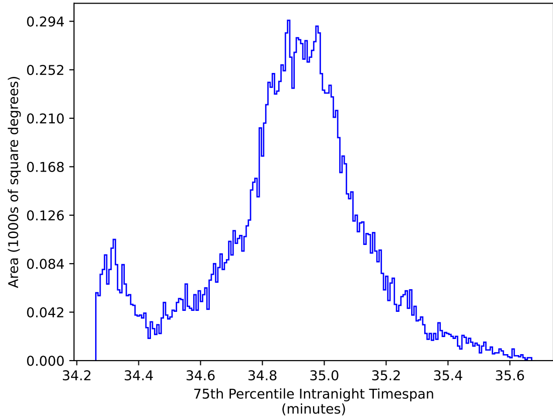
too_elab_heavy_r32_d3_ugrizy_v3.4_10yrs WFD all bands: 75th Percentile Intranight Timespan
