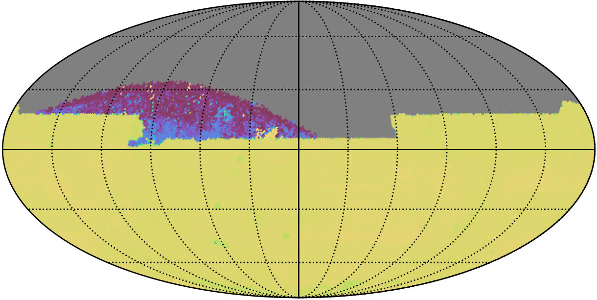
too_elab_heavy_r32_d3_ugrizy_v3.4_10yrs All sky zy bands: 75th Percentile Intranight Timespan
