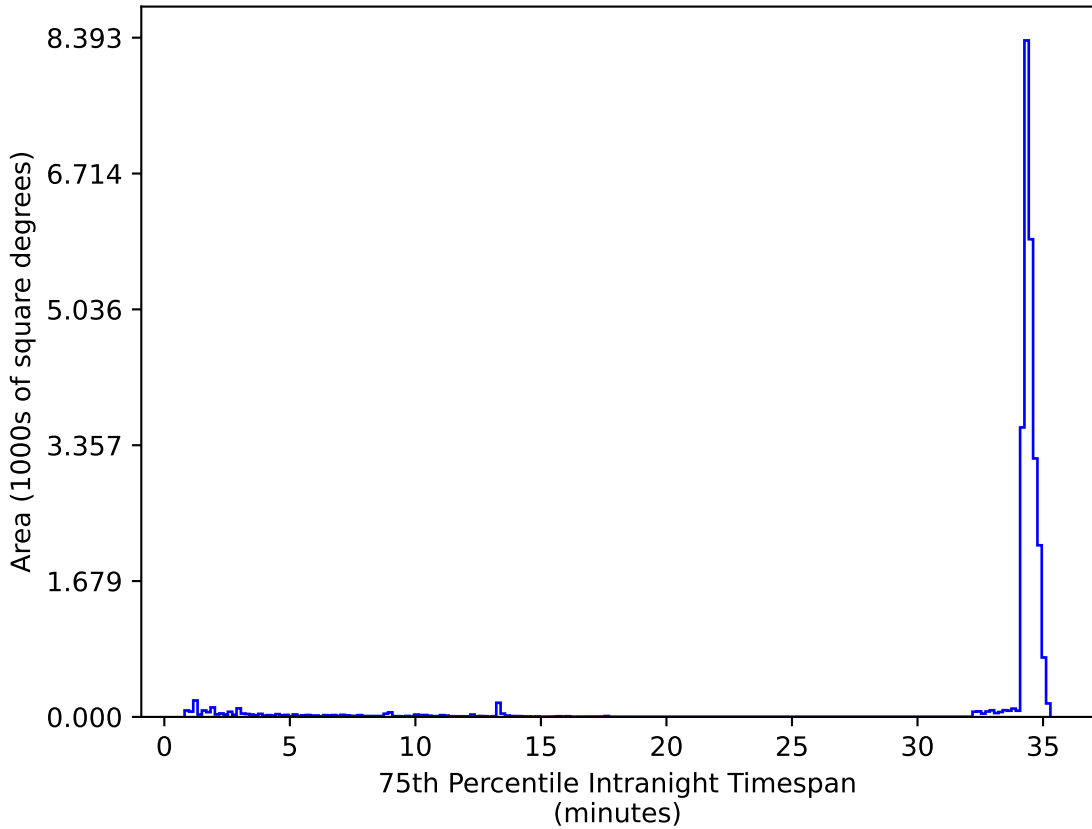
too_elab_heavy_r32_d3_ugrizy_v3.4_10yrs All sky zy bands: 75th Percentile Intranight Timespan
