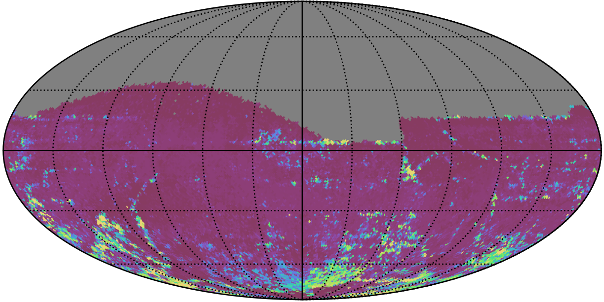
too_elab_heavy_r32_d3_ugrizy_v3.4_10yrs All sky z band: 75th Percentile Intranight Timespan
