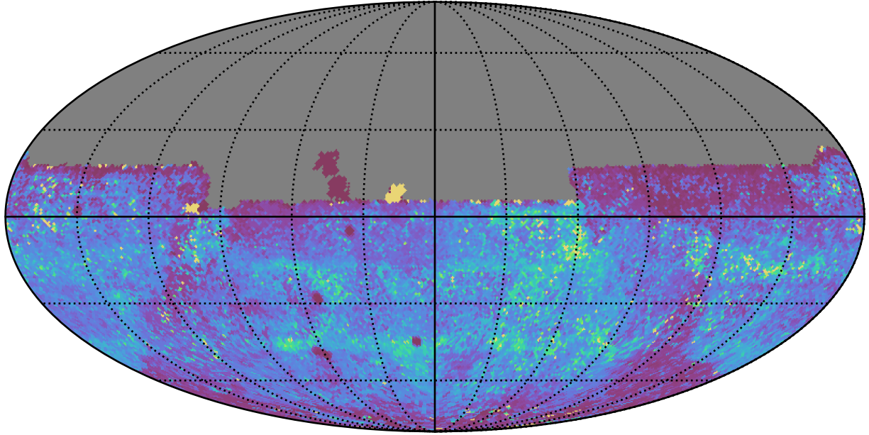
too_elab_heavy_r32_d3_ugrizy_v3.4_10yrs All sky y band: 75th Percentile Intranight Timespan
