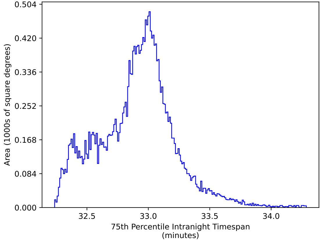
too_elab_heavy_r32_d3_ugrizy_v3.4_10yrs All sky y band: 75th Percentile Intranight Timespan
