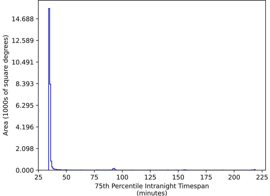
too_elab_heavy_r32_d3_ugrizy_v3.4_10yrs All sky ri bands: 75th Percentile Intranight Timespan
