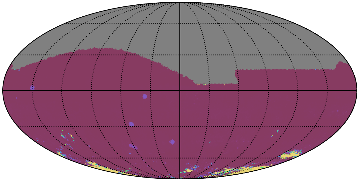
too_elab_heavy_r32_d3_ugrizy_v3.4_10yrs All sky iz bands: 75th Percentile Intranight Timespan
