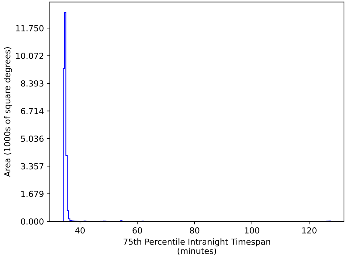
too_elab_heavy_r32_d3_ugrizy_v3.4_10yrs All sky iz bands: 75th Percentile Intranight Timespan
