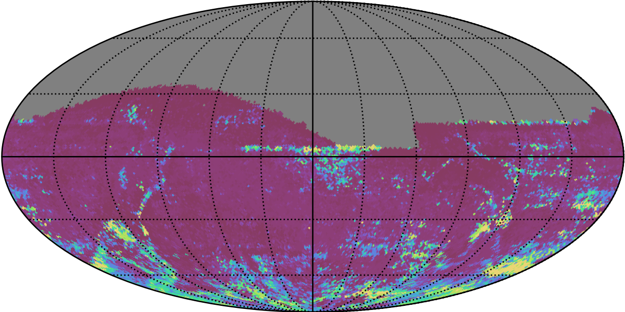
too_elab_heavy_r32_d3_ugrizy_v3.4_10yrs All sky i band: 75th Percentile Intranight Timespan
