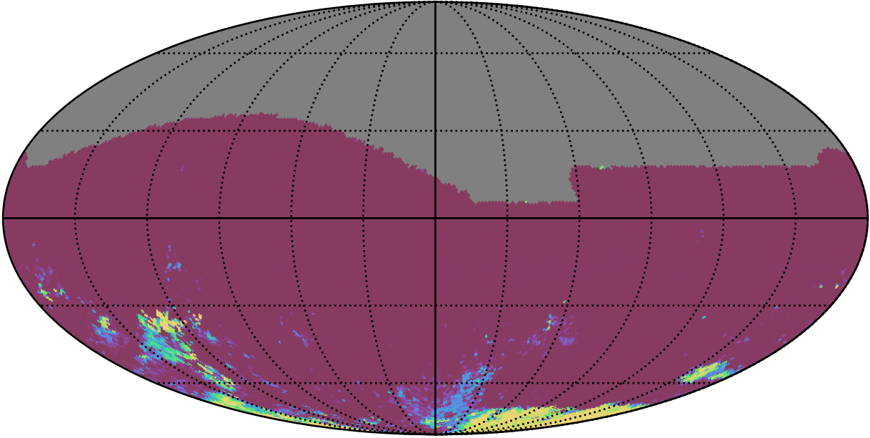
too_elab_heavy_r32_d3_ugrizy_v3.4_10yrs All sky gr bands: 75th Percentile Intranight Timespan
