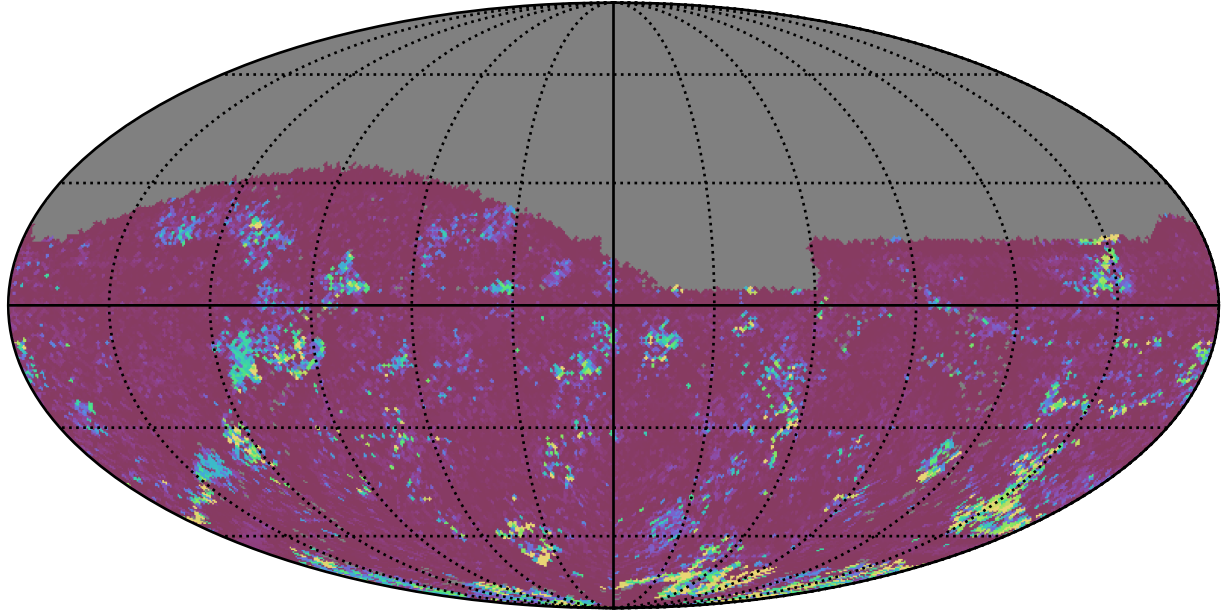
too_elab_heavy_r32_d3_ugrizy_v3.4_10yrs All sky g band: 75th Percentile Intranight Timespan
