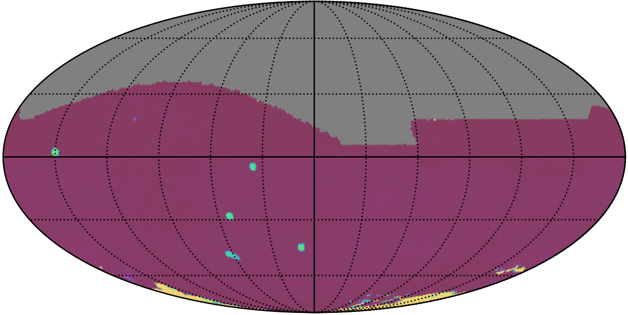
too_elab_heavy_r32_d3_ugrizy_v3.4_10yrs All sky all bands: 75th Percentile Intranight Timespan
