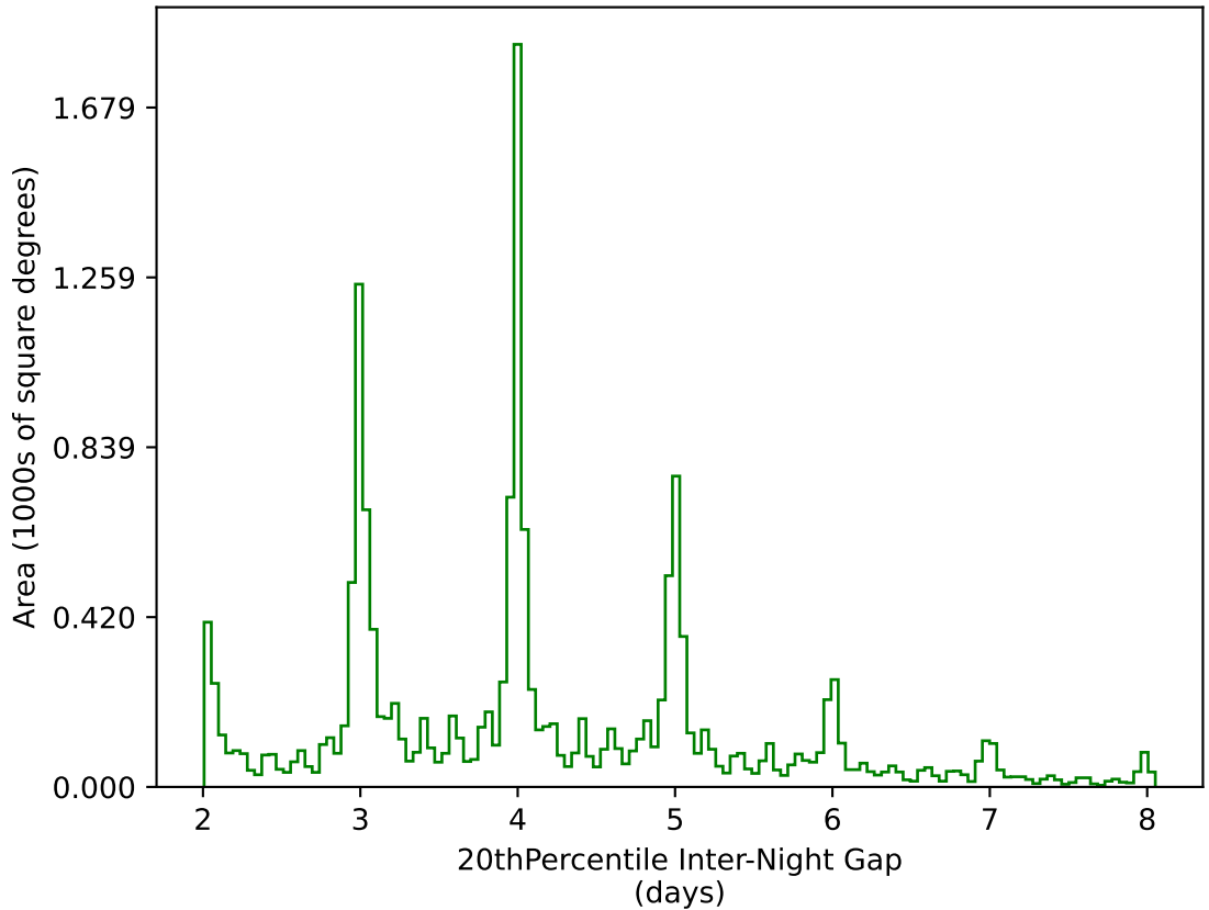
too_elab_heavy_r32_d3_ugrizy_v3.4_10yrs WFD g band: 20thPercentile Inter-Night Gap
