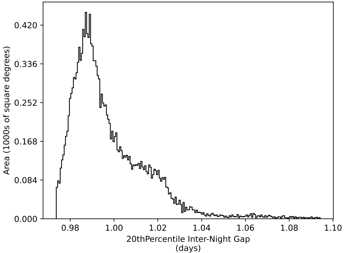
too_elab_heavy_r32_d3_ugrizy_v3.4_10yrs WFD all bands: 20thPercentile Inter-Night Gap
