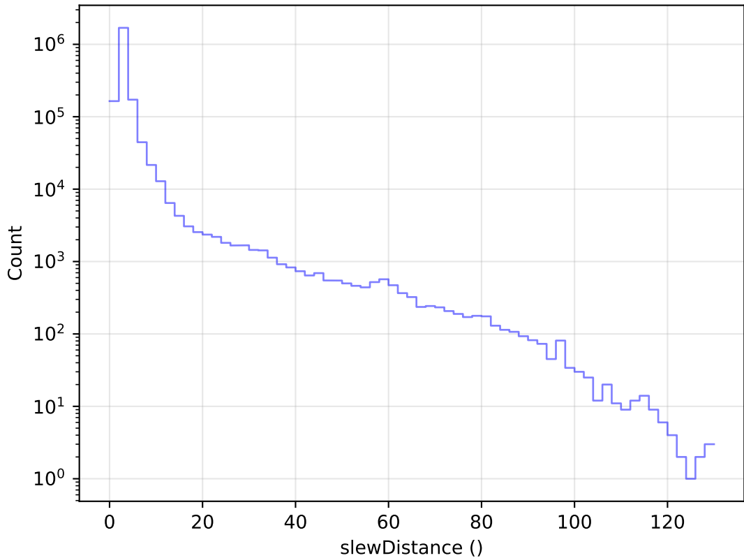
too_elab_heavy_r32_d3_ugrizy_v3.4_10yrs All visits: Slew Distance Histogram
