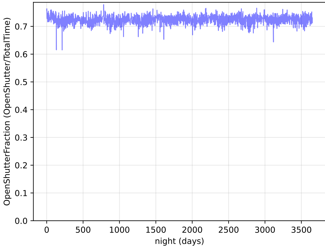
too_elab_heavy_r32_d3_ugrizy_v3.4_10yrs : OpenShutterFraction
