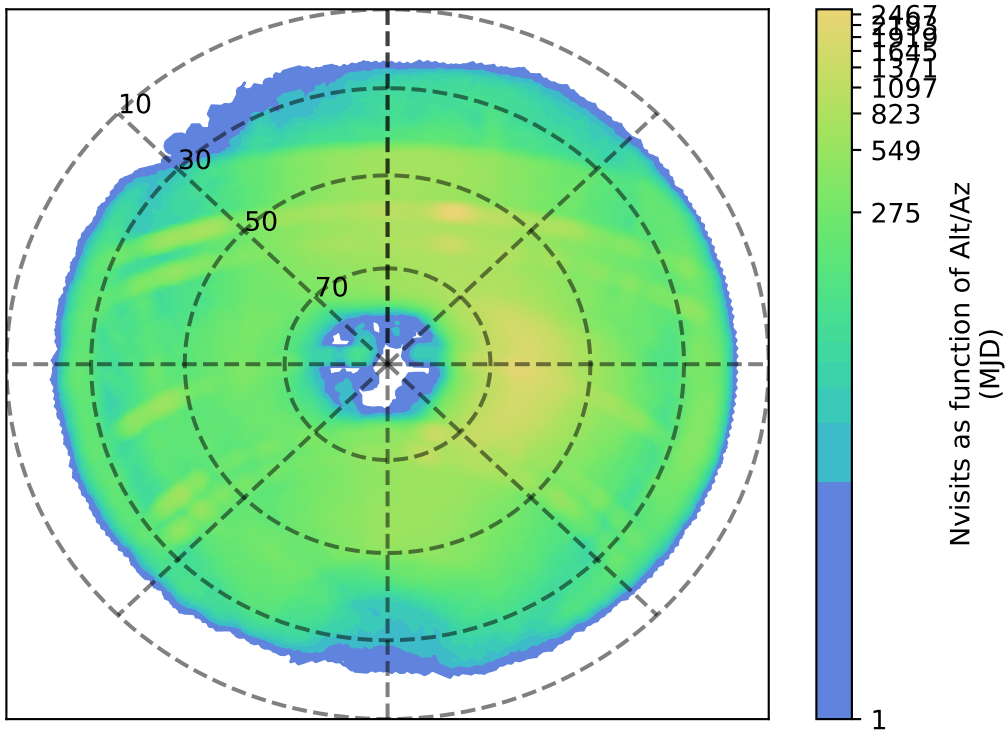
too_elab_heavy_r32_d3_ugrizy_v3.4_10yrs z: Nvisits as function of Alt/Az
