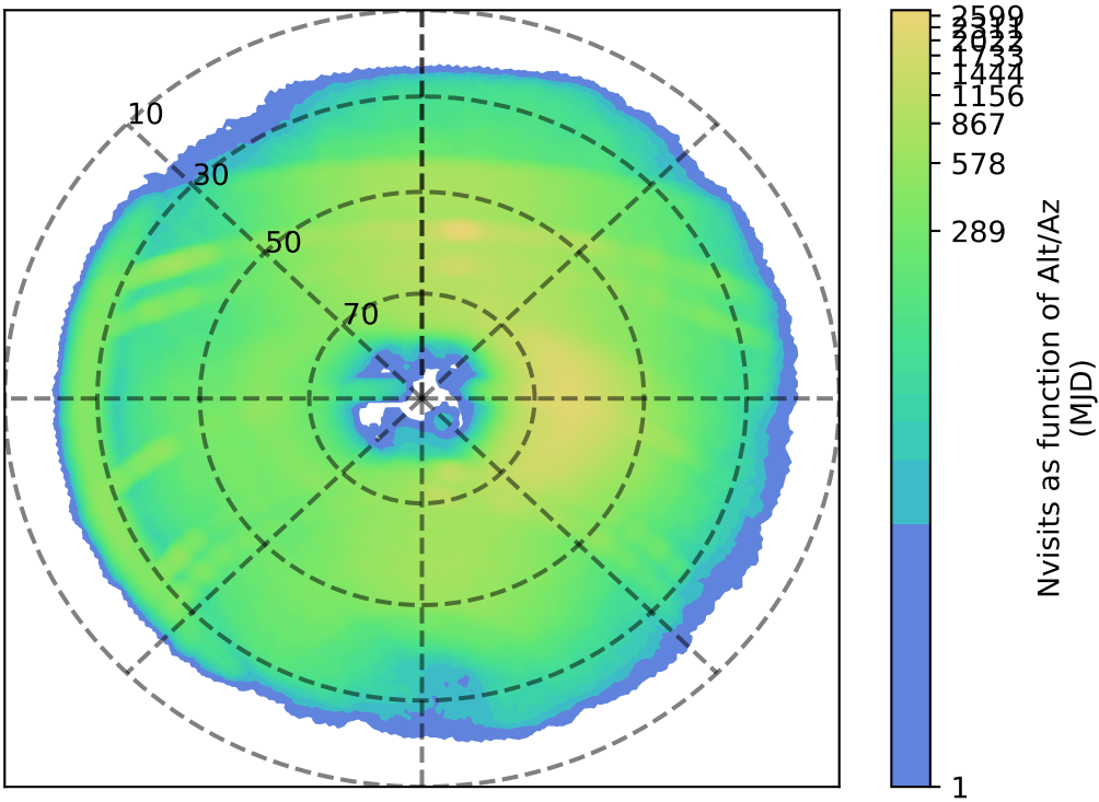
too_elab_heavy_r32_d3_ugrizy_v3.4_10yrs r: Nvisits as function of Alt/Az
