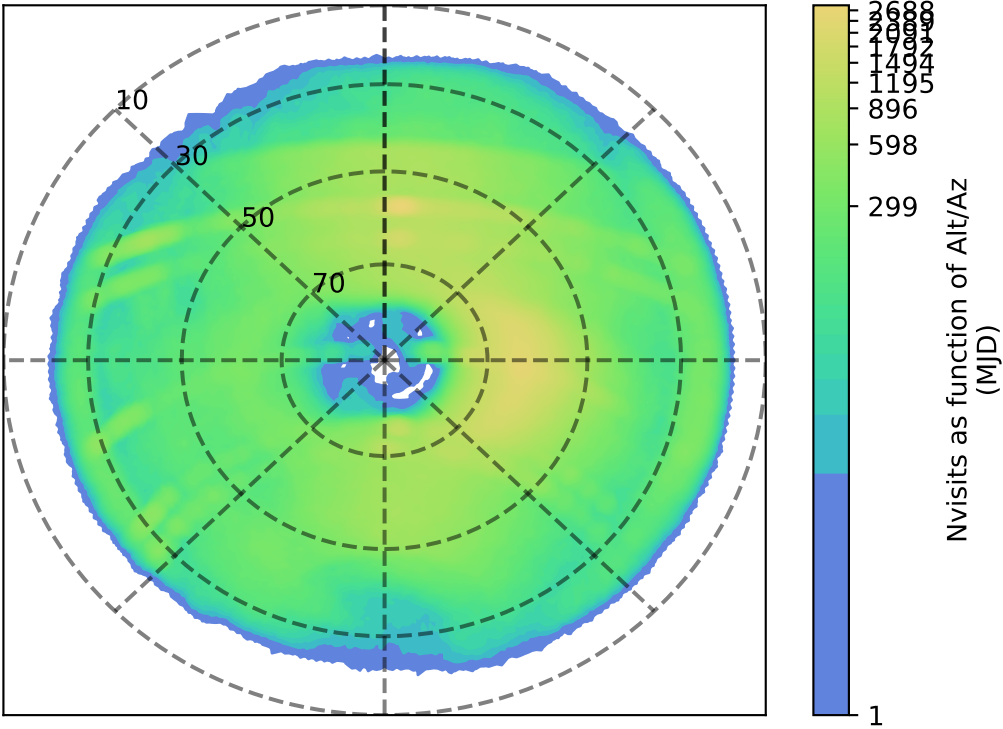
too_elab_heavy_r32_d3_ugrizy_v3.4_10yrs i: Nvisits as function of Alt/Az
