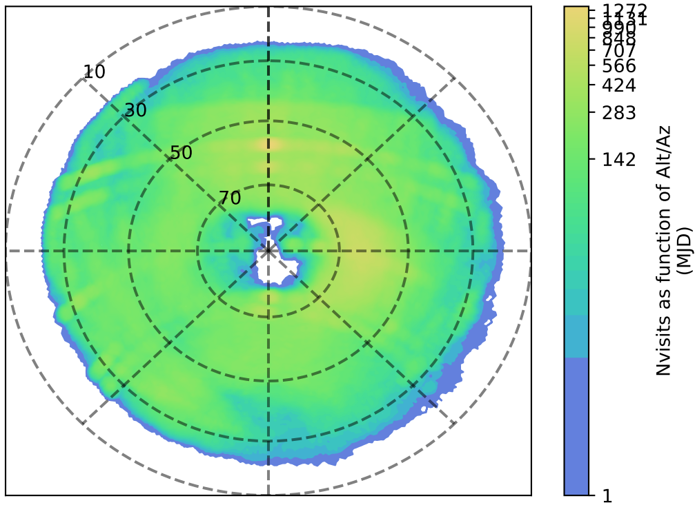
too_elab_heavy_r32_d3_ugrizy_v3.4_10yrs g: Nvisits as function of Alt/Az
