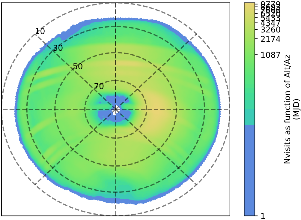
too_elab_heavy_r32_d3_ugrizy_v3.4_10yrs : Nvisits as function of Alt/Az
