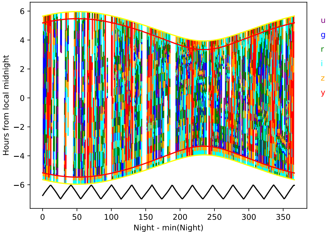
too_elab_heavy_r32_d3_ugrizy_v3.4_10yrs year 0-1: Hourglass
