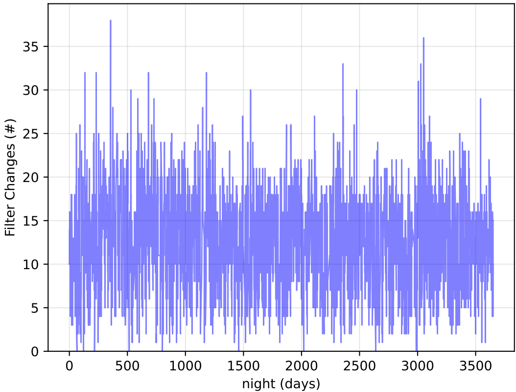
too_elab_heavy_r32_d3_ugrizy_v3.4_10yrs : Filter Changes
