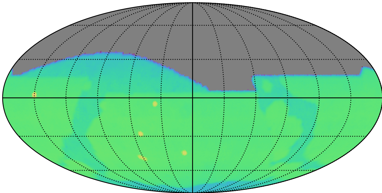
too_elab_heavy_r32_d3_ugrizy_v3.4_10yrs : CoaddM5
