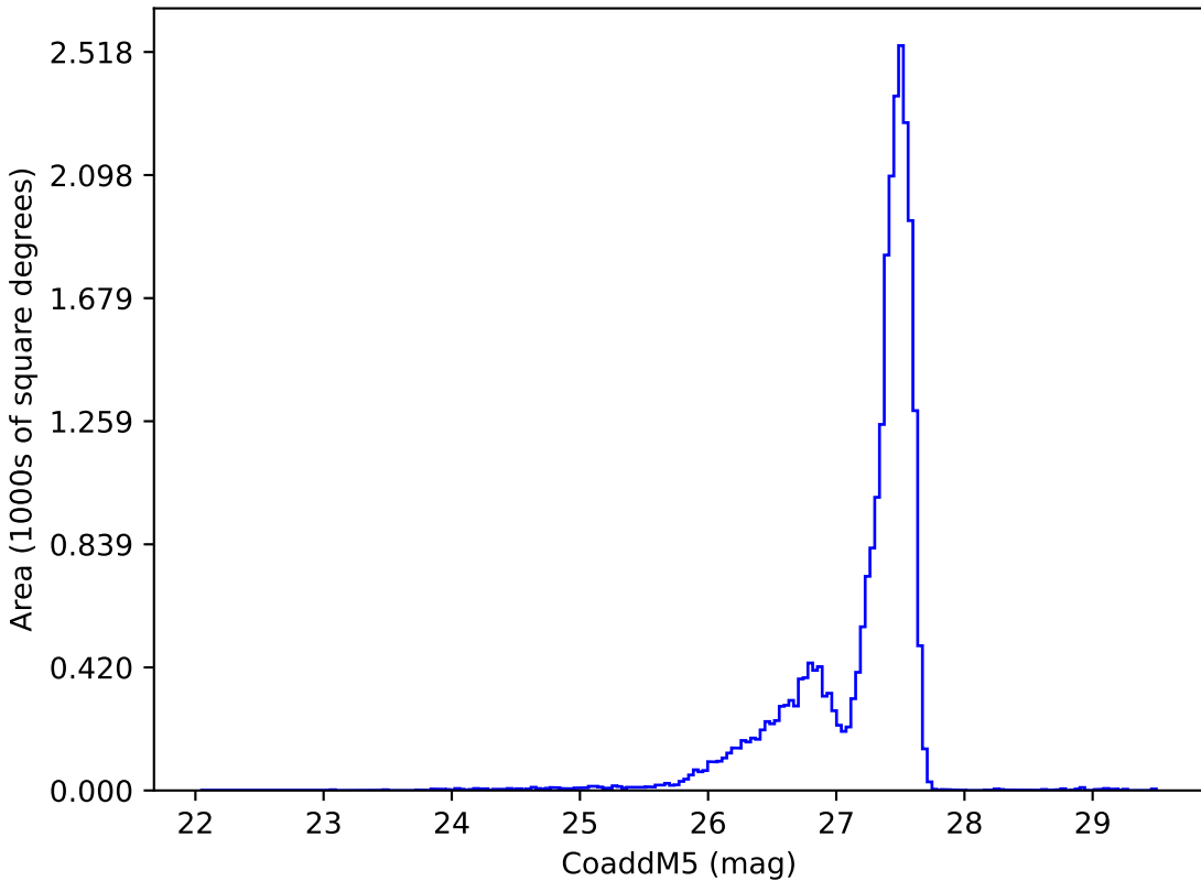
too_elab_heavy_r32_d3_ugrizy_v3.4_10yrs : CoaddM5
