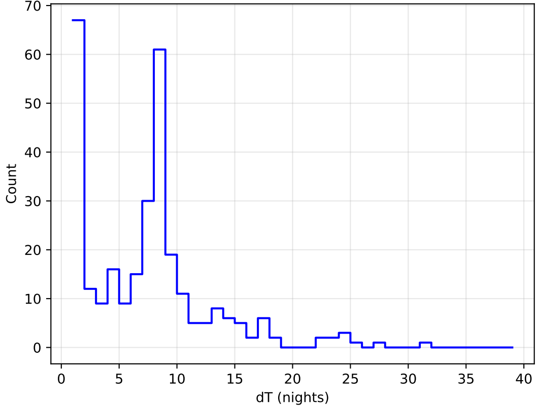
too_elab_heavy_r32_d3_ugrizy_v3.4_10yrs all bands: DD:XMM_LSS Delta Nights Histogram
