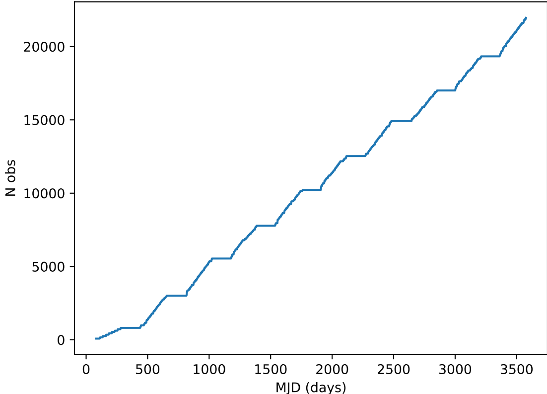
too_elab_heavy_r32_d3_ugrizy_v3.4_10yrs all bands: DD:XMM_LSS Cumulative NVisits
