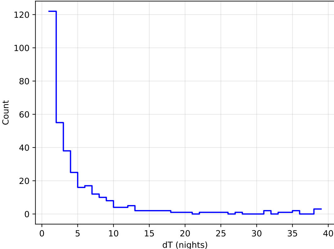
too_elab_heavy_r32_d3_ugrizy_v3.4_10yrs all bands: DD:WFD Delta Nights Histogram
