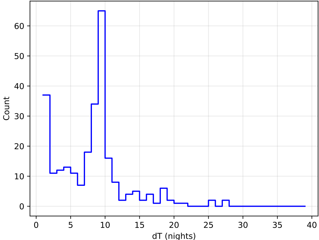
too_elab_heavy_r32_d3_ugrizy_v3.4_10yrs all bands: DD:ELAISS1 Delta Nights Histogram
