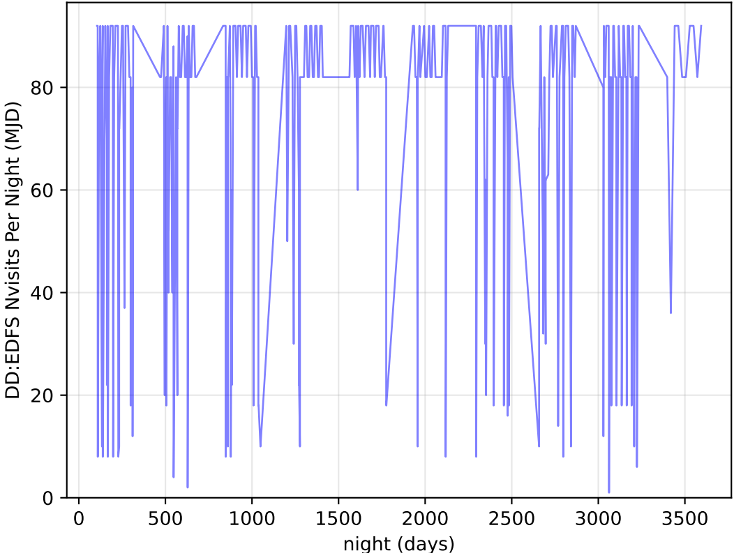
too_elab_heavy_r32_d3_ugrizy_v3.4_10yrs all bands: DD:EDFS Nvisits Per Night
