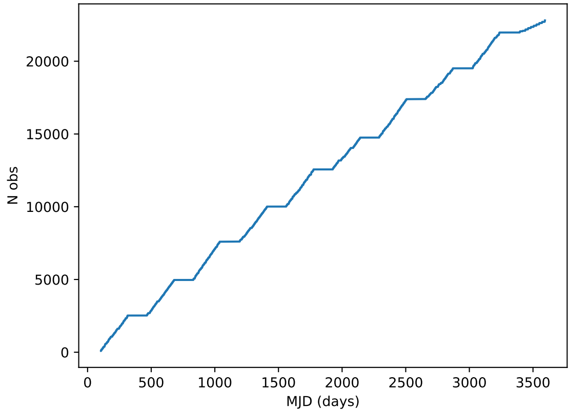
too_elab_heavy_r32_d3_ugrizy_v3.4_10yrs all bands: DD:EDFS Cumulative NVisits
