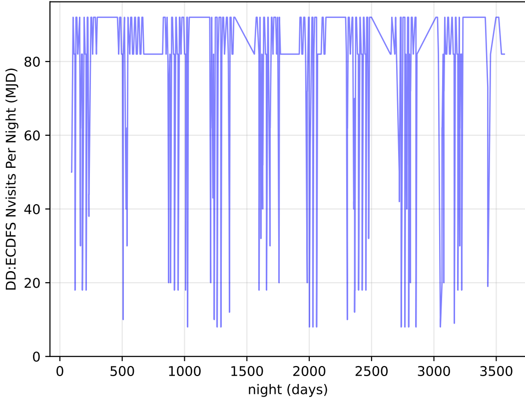
too_elab_heavy_r32_d3_ugrizy_v3.4_10yrs all bands: DD:ECDFS Nvisits Per Night
