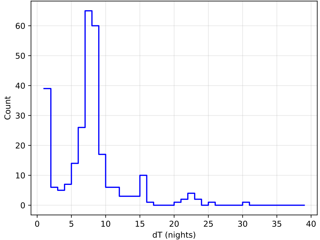
too_elab_heavy_r32_d3_ugrizy_v3.4_10yrs all bands: DD:ECDFS Delta Nights Histogram
