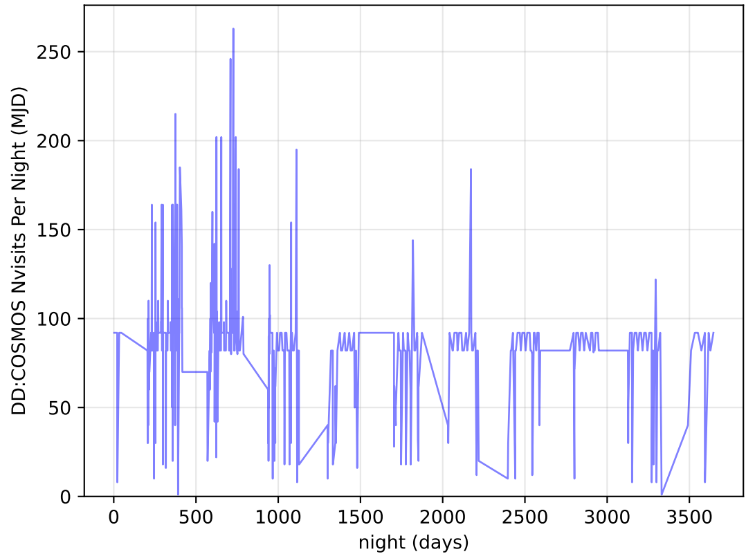
too_elab_heavy_r32_d3_ugrizy_v3.4_10yrs all bands: DD: COSMOS Nvisits Per Night
