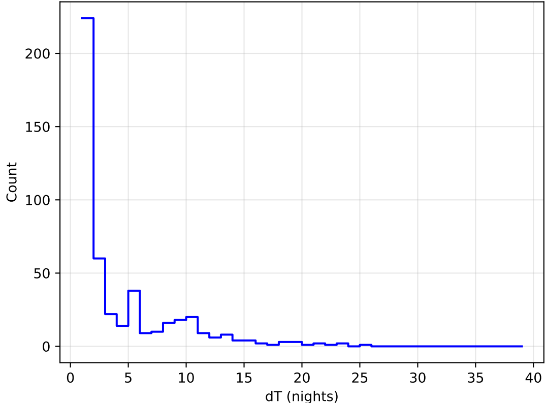
too_elab_heavy_r32_d3_ugrizy_v3.4_10yrs all bands: DD: COSMOS Delta Nights Histogram
