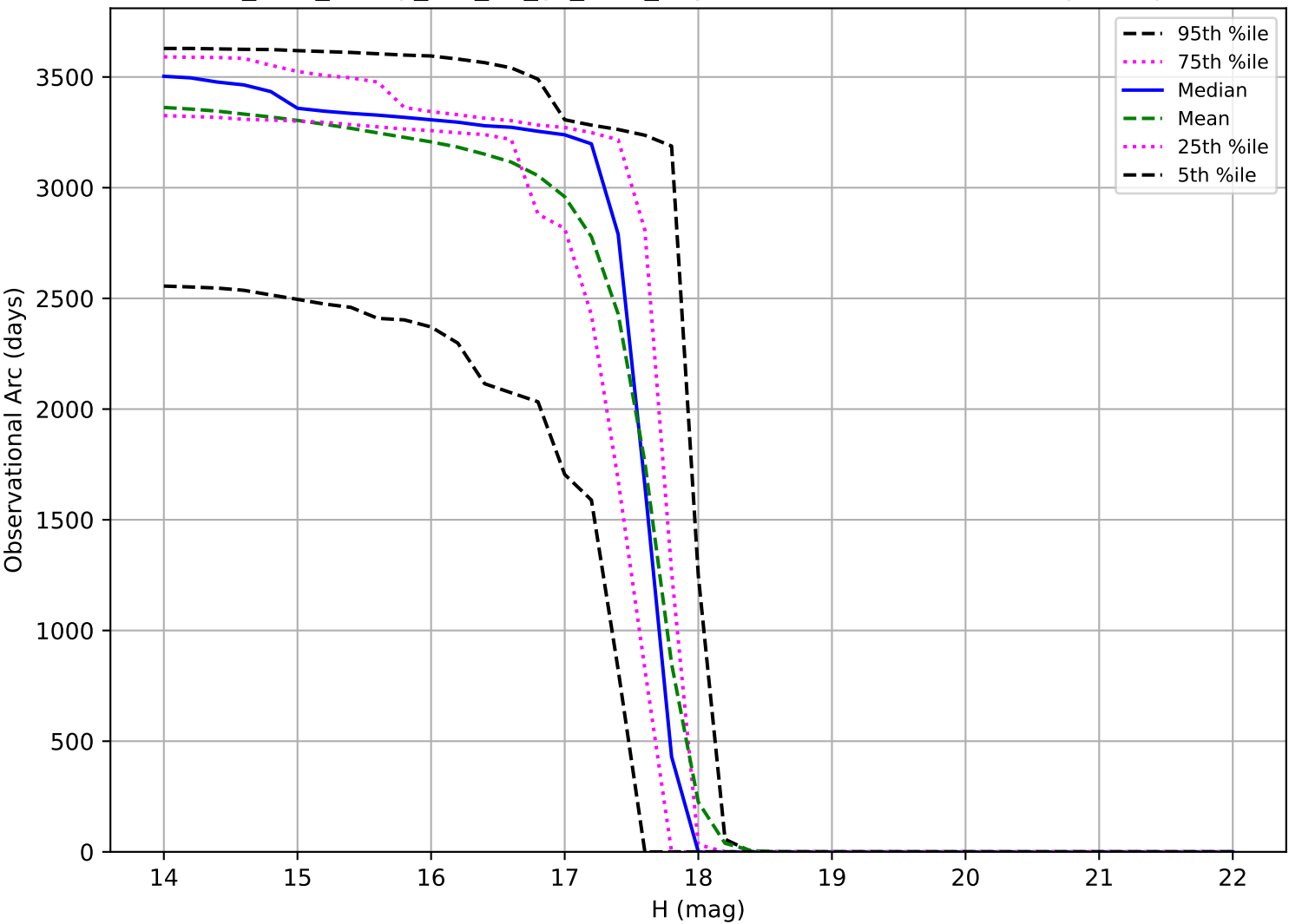
too_elab_heavy_r32_d3_gz_v3.4_10yrs: Observational Arc Length Trojan
