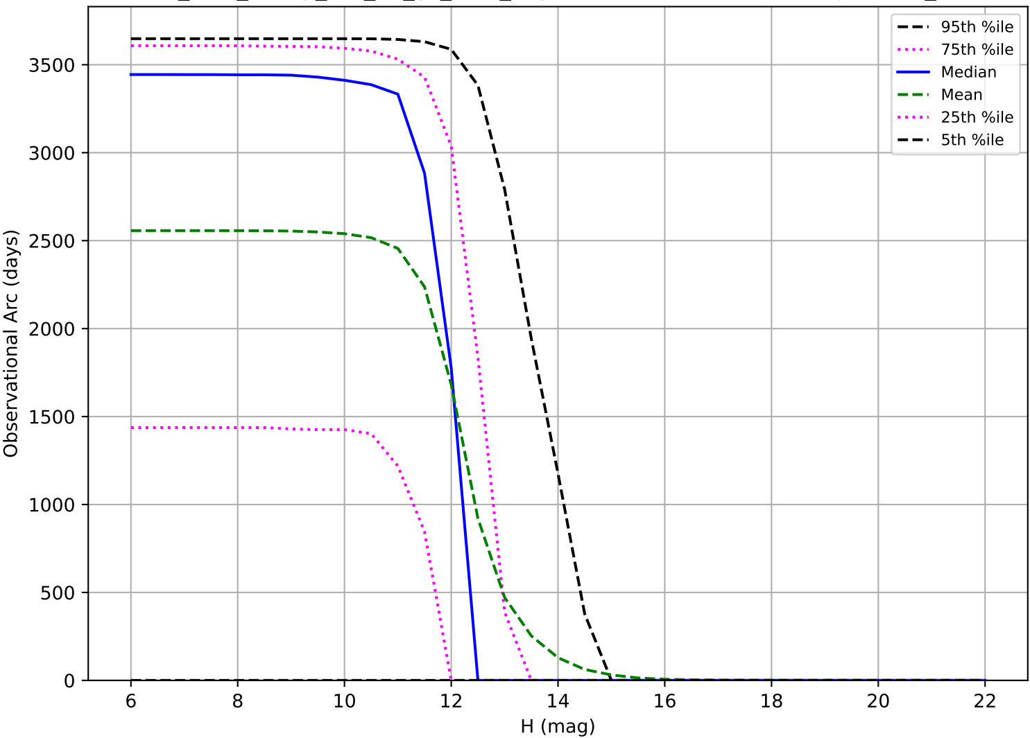
too_elab_heavy_r32_d3_gz_v3.4_10yrs: Observational Arc Length OCC_r20
